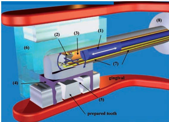
Fig. 6: Intraoral microscanner: probe (1), mirror (2), water supply (3), connection (4), gel coupling (5), bite splint as counter bearing (6), micro-mechanics (7,8)
